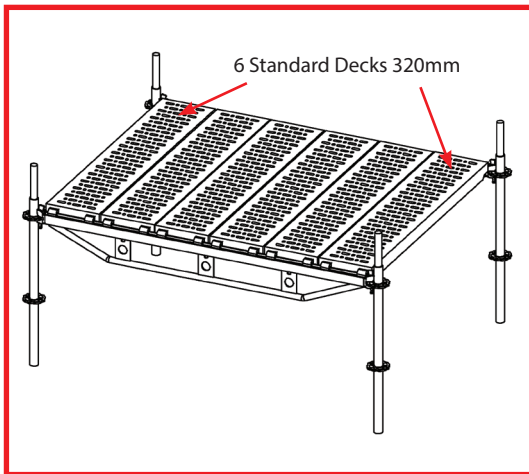
Figure 28: The 2.07m wide bay
