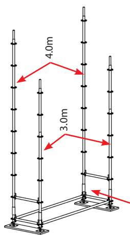
Figure 7: Assembly of the vertical standards
