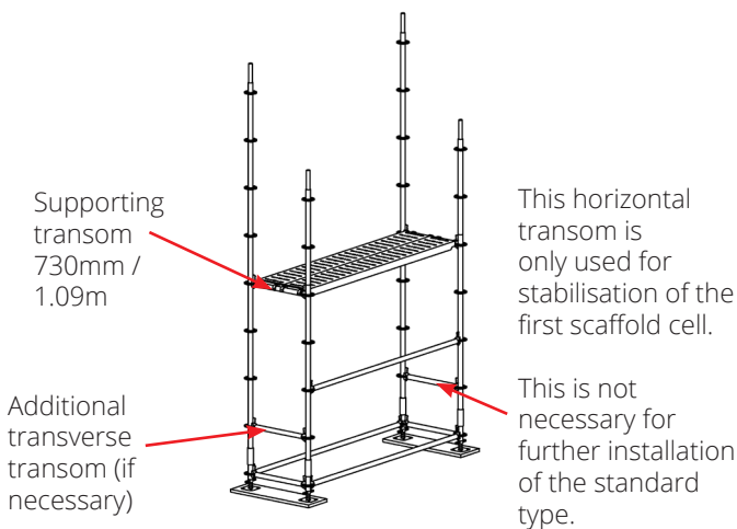
Figure 8: Assembly of the deck
