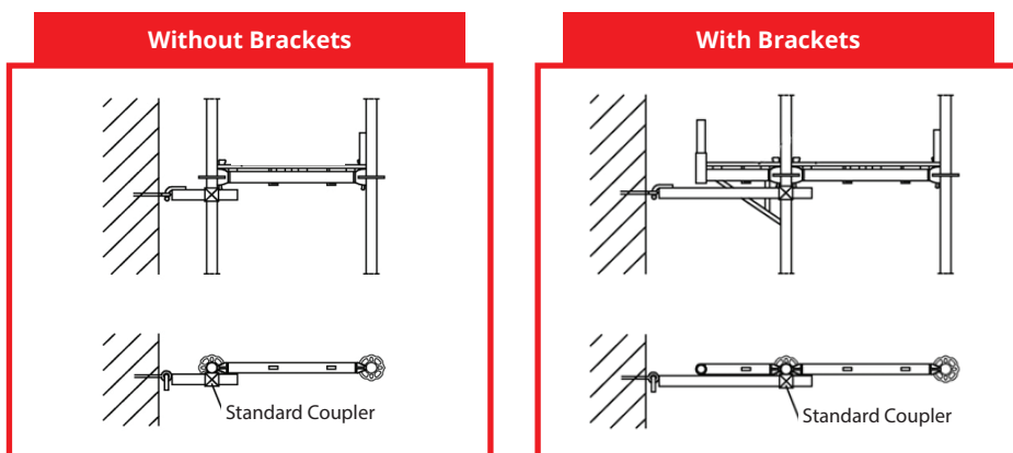
Figure 21: Short scaffold brackets
