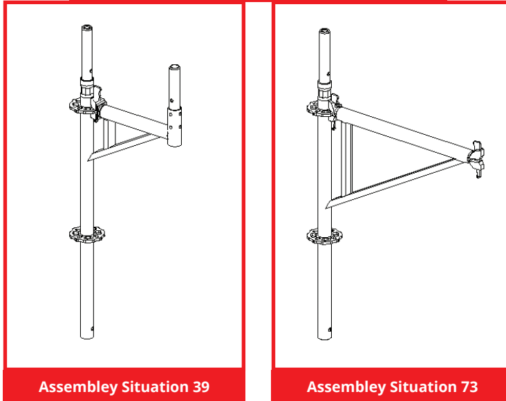
Figure 37: Adjustable bracket 39/73 (tube support)
