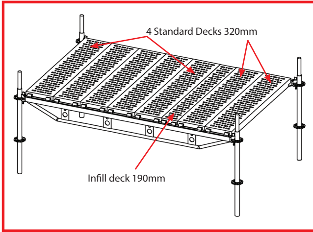
Figure 29: The 2.57m wide bay
