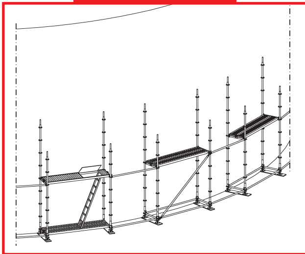
Figure 45: Lower Scaffold Level
