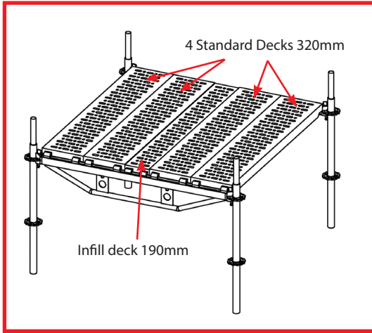
Figure 27: The 1.57m wide bay
