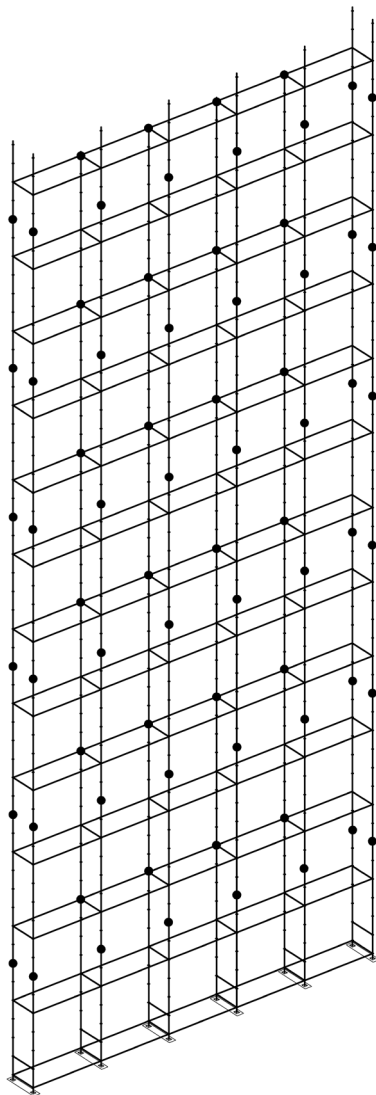
Figure 16: Position of the post butt joints.
