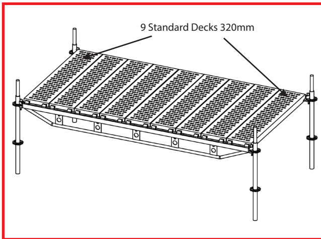
Figure 30: The 3.07m wide bay
