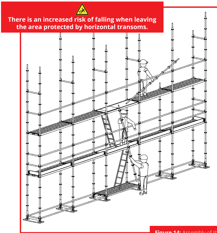
Figure 14: Assembly of the vertical standards.
